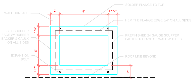
SCUPPER - TYP. EXT. ELEVATION NOT TO SCALE
