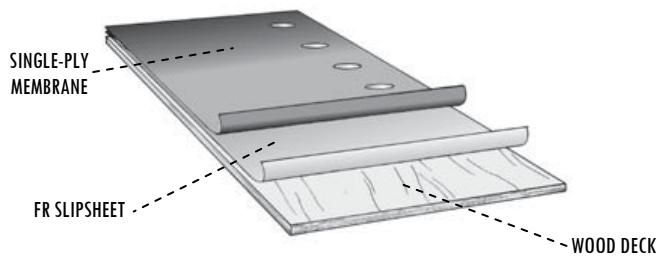
TYPICAL COMBUSTIBLE DECK APPLICATION
