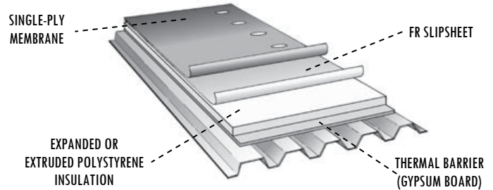
TYPICAL STEEL DECK & POLYSTYRENE INSULATION
