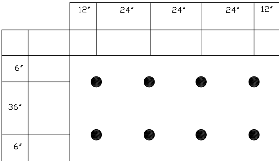
4' X 8' FLEX INSULATION OR RECOVER BOARD 8 FLEX PLATES AND FASTENERS PER BOARD
