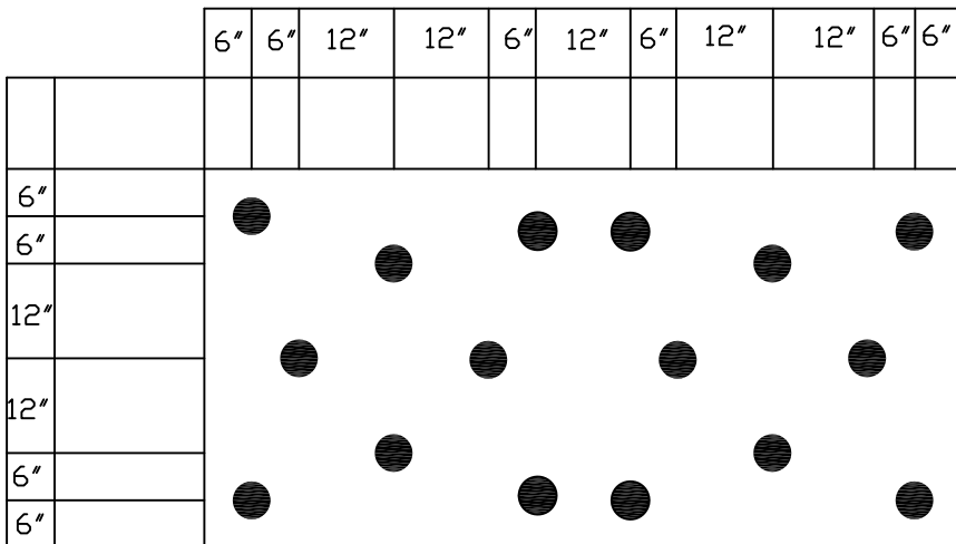
4' X 8' FLEX INSULATION OR RECOVER BOARD 16 FLEX PLATES AND FASTENERS PER BOARD
