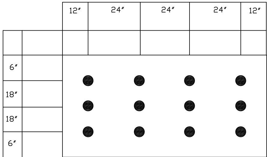
4' X 8' FLEX INSULATION OR RECOVER BOARD 12 FLEX PLATES AND FASTENERS PER BOARD
