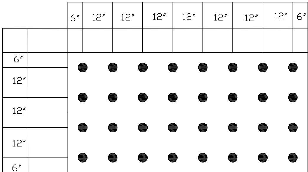
4' X 8' FLEX INSULATION OR RECOVER BOARD 32 FLEX PLATES AND FASTENERS PER BOARD
