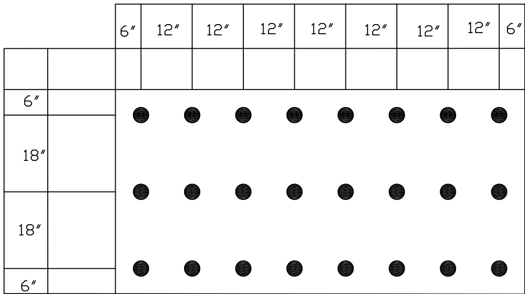
4' X 8' FLEX INSULATION OR RECOVER BOARD 24 FLEX PLATES AND FASTENERS PER BOARD
