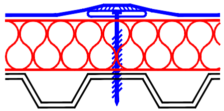
FLEX FASTENER AND ISOWELD PLATE
