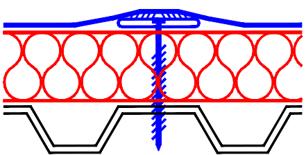
FLEX FASTENER AND ISOWELD PLATE
