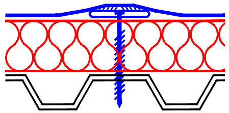
FLEX FASTENER AND RHINO BOND PLATE
